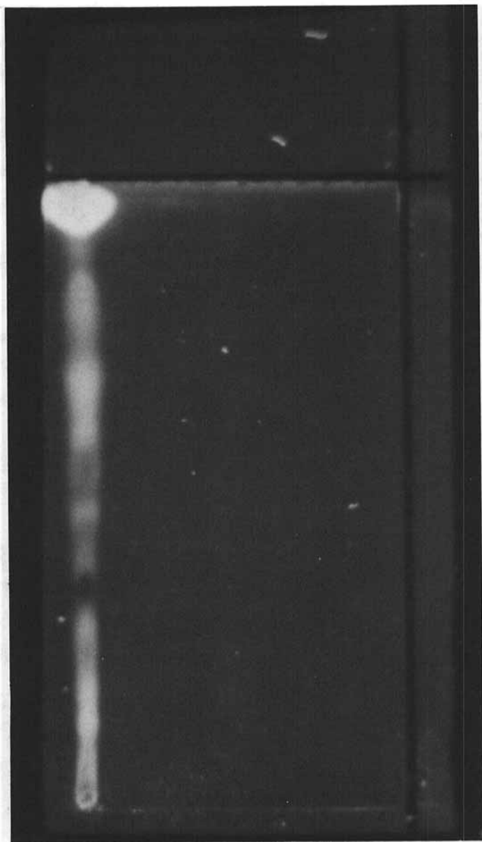
Fig. 1. One-dimensional development with acetone—chloroform showing no separation of aflatoxins from interfering substances. The corn sample contained naturally occurring aflatoxin B 1 and was spiked with 20 ppb each of B 1 , B 2 , G 1 , and G 2 .
