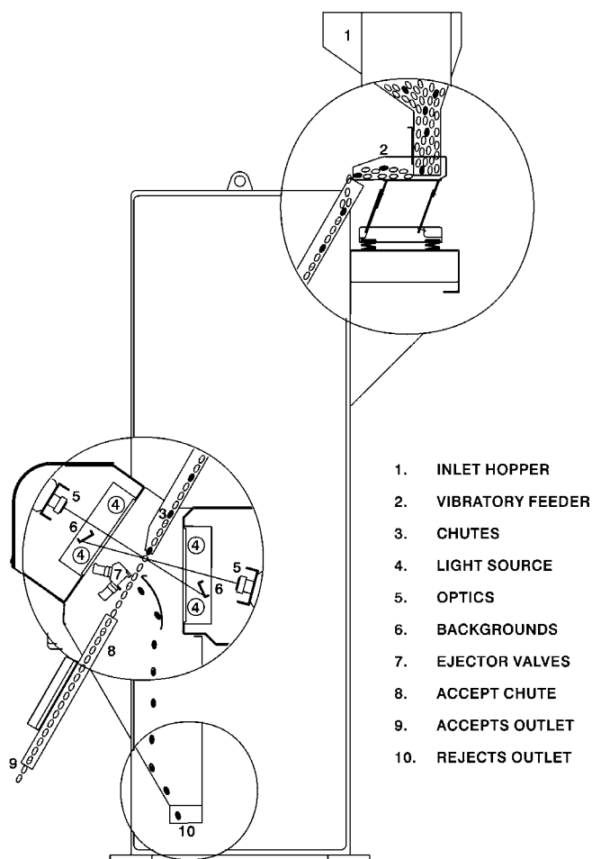
Fig. 1. Side view and cut-away sections of high-volume color sorter. Computer screen is in front.
