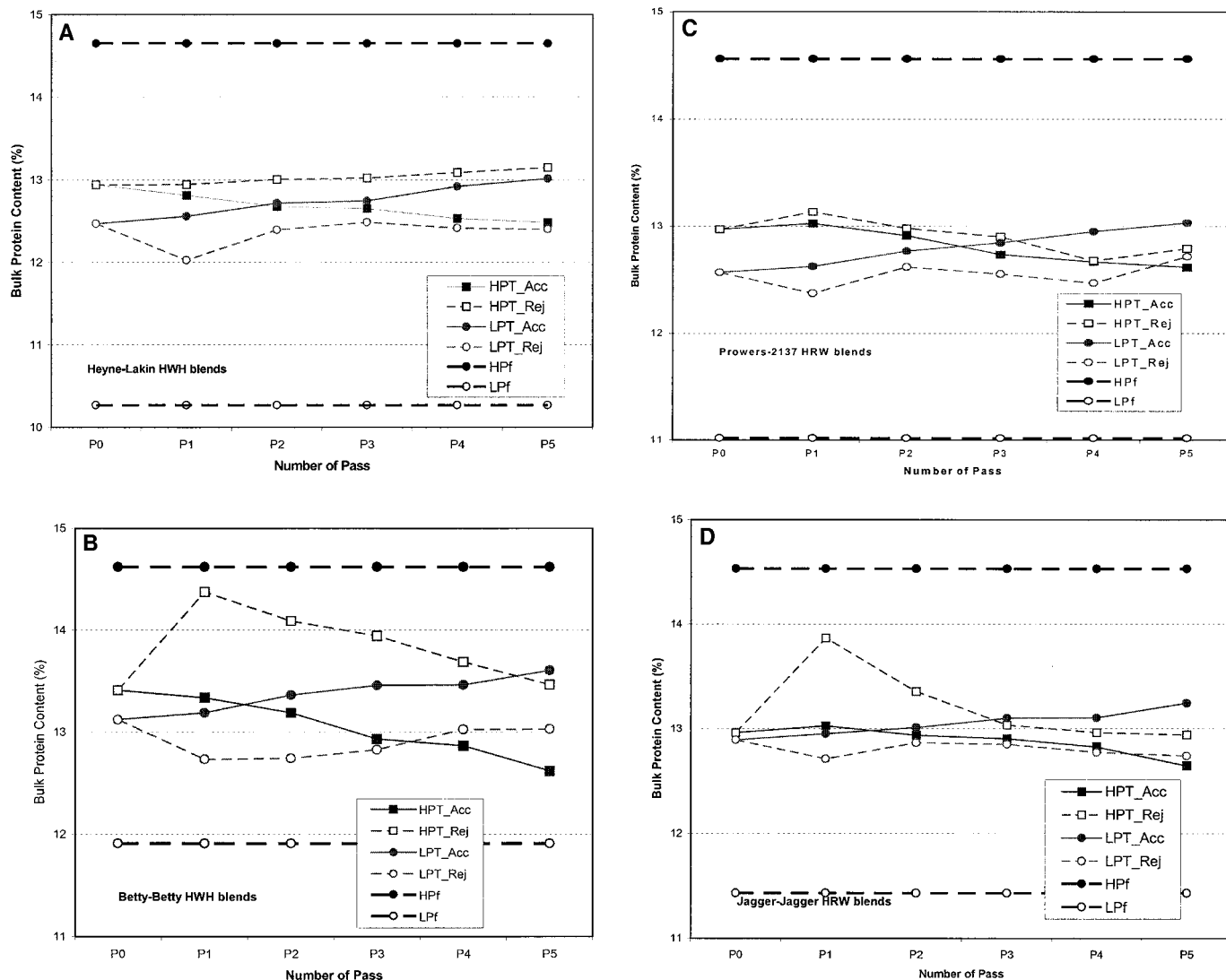
Fig. 2. Bulk protein content of accepted and rejected kernels for each pass, for high- and low-protein thresholds, for the four wheat blends used (white background). HPT_Acc, kernels accepted by high-protein threshold; HPT_rej, kernels rejected by high-protein threshold; LPT_Acc, kernels accepted by low-protein threshold; LPT_rej, kernels rejected by low-protein threshold; HPf, high-protein fraction of the blend; LPf, low-protein fraction of the blend.
