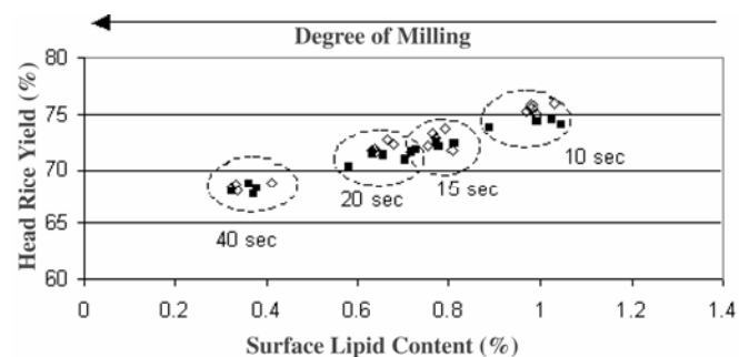
Fig. 3. Effect of surface lipid content (SLC) on head rice yield (HRY) of Bengal rice grown in 2004 in Jonesboro, AR (◇) and Lodge Corner, AR (■). Circled data points represent rice milled for 10, 15, 20, 40 sec, with degree of milling increasing with decreasing SLC. Each point is the mean HRY and SLC of duplicate samples milled after 0, 1, 2, 3, or 6 months of storage.
