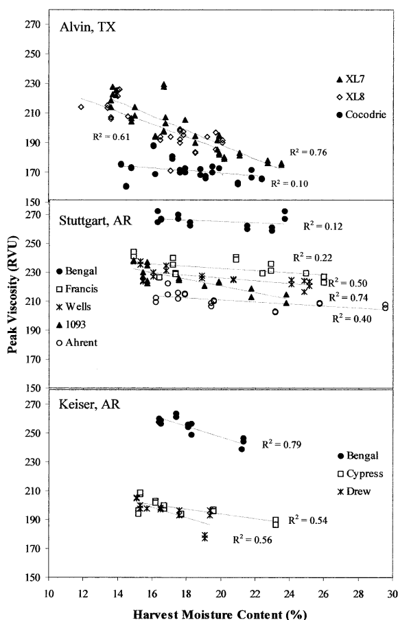
Fig. 2. Effects of harvest moisture content (wb) on peak viscosity of rice cultivars from Alvin, TX, and Stuttgart and Keiser, AR, in 2002.
