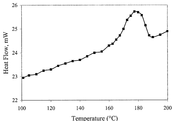
Fig. 2. Differential scanning calorimetry thermogram at 100\text{--}200^\circ\text{C} for coarsely ground brown rice kernels (cv. Drew, 14% moisture content).
