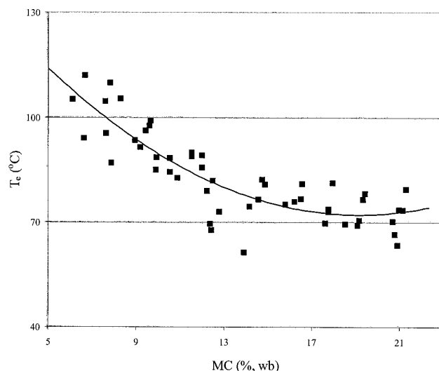
Fig. 8. Rapid evaporation temperature ( T_c ) as a function of moisture content for brown rice kernels (cv. Drew).
