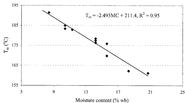
Fig. 3. Melting temperature ( T_m ) of coarsely ground brown rice kernels (cv. Drew) as a function of moisture content.
