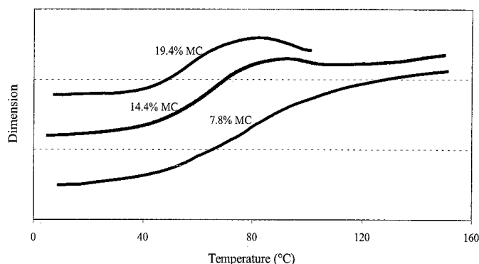
Fig. 5. Thermomechanical analysis curves for brown rice kernels (cv. Drew) at different moisture contents. Distance between two dashed lines on the y axis is 0.01 mm.
