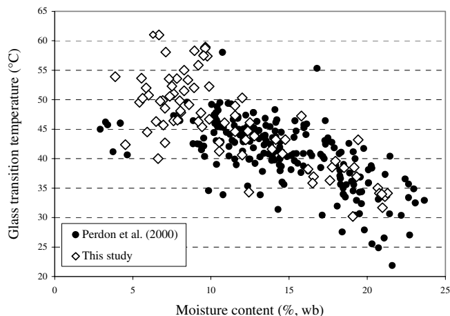
Fig. 7. Glass transition temperature vs. moisture content for brown rice kernels (cv. Drew in this study; cvs. Bengal and Cypress in Perdon et al [2000]).
