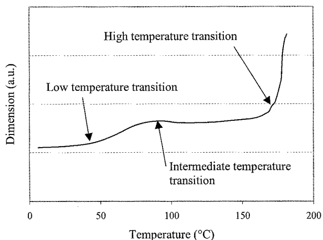
Fig. 1. Thermomechanical analysis curve for a brown rice kernel (cv. Drew, 14.4% moisture content). On the y axis, a.u. stands for arbitrary unit.
