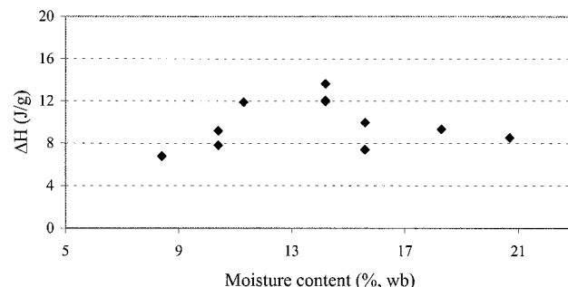
Fig. 4. Melting enthalpy ( \Delta H ) of coarsely ground brown rice kernels (cv. Drew) in relation to moisture content.
