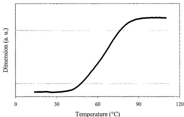
Fig. 6. Thermomechanical analysis curve for rice starch at 10.4% moisture content.
