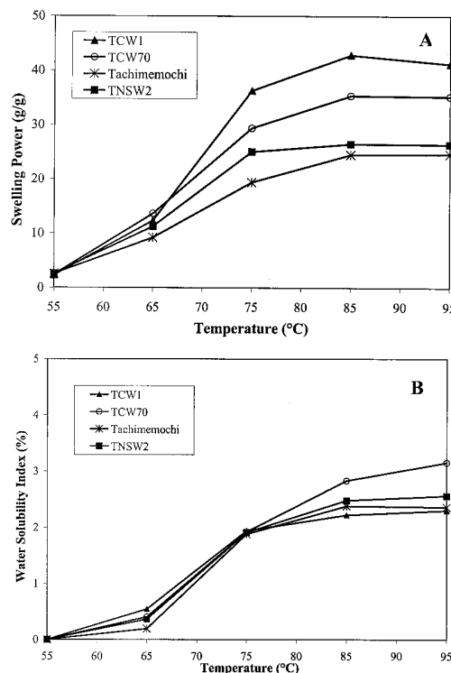
Fig. 2. Swelling power (A) and water solubility index (B) of waxy rice starches.
