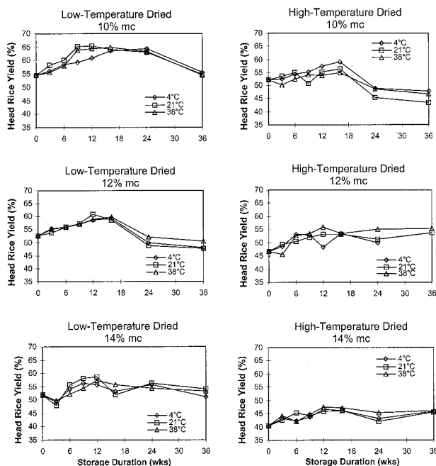
Fig. 1. Head rice yield as a function of rough rice storage duration and temperature for low- and high-temperature-dried rice (cv. Kaybonnet) stored at 10, 12, and 14% moisture content.
