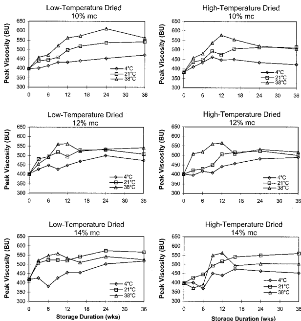
Fig. 3. Peak viscosity as a function of rough rice storage duration and temperature for low- and high-temperature-dried rice (cv. Kaybonnet) stored at 10, 12, and 14% moisture content.
