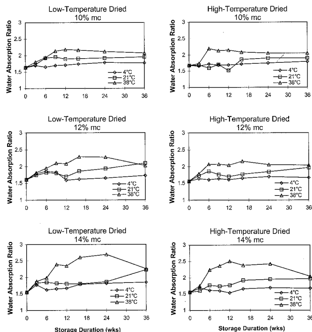
Fig. 2. Water absorption ratios as a function of rough rice storage duration and temperature for low- and high-temperature-dried rice (cv. Kaybonnet) stored at 10, 12, and 14% moisture content.
