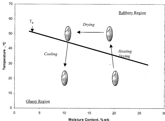
Fig. 6. Brown rice state diagram (Bengal and Cypress data combined) and a hypothetical drying process for a rice kernel.
