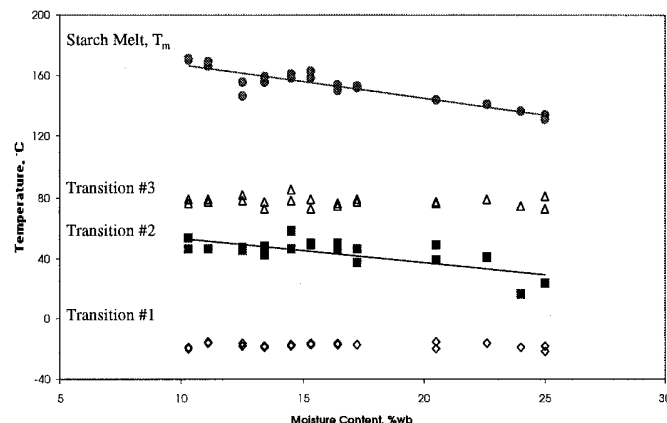
Fig. 3. Thermal transitions determined from differential scanning calorimetry (DSC) of Bengal brown rice kernels at different MC.
