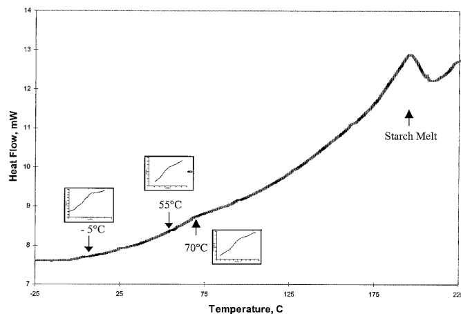
Fig. 2. Differential scanning calorimetry (DSC) thermogram of Bengal brown rice at 12% MC. Multiple transitions (slope change in heat capacity) at different temperatures indicated by arrows.
