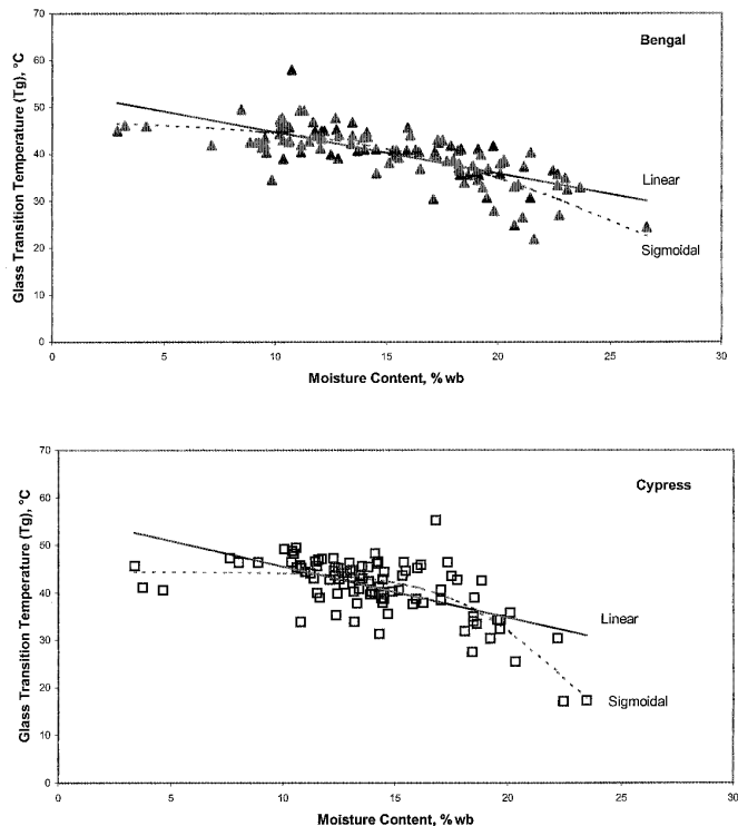
Fig. 5. Linear and sigmoidal models (see Table IV) for Bengal and Cypress brown rice state diagrams.
