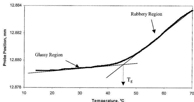
Fig. 1. Typical thermomechanical analysis (TMA) thermogram indicating assignment of glass transition temperature ( T_g ) and glassy and rubbery regions.
