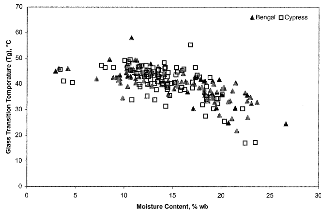
Fig. 4. Glass transition temperatures measured with thermomechanical analysis (TMA) of individual brown rice kernels of Bengal and Cypress, plotted against corresponding MC.
