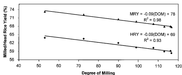
Fig. 3. A typical plot of milled rice yield (MRY) and head rice yield (HR Y) vs. degree of milling (DOM), as measured with a Satake MM1-B milling meter.
