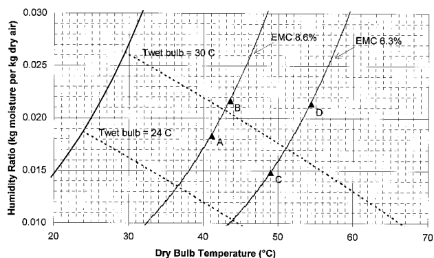
Fig. 1. Psychrometric representation of four (A–D) drying conditions. Equilibrium moisture contents (EMC) were calculated according to the Chung equation (ASAE 1995).
