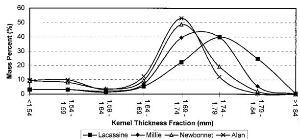
Fig. 5. Mass percentages of kernel thickness fractions for rice cultivars.
