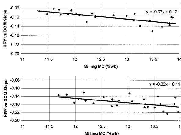
Fig. 2. Head rice yield (HRY) vs. degree of milling (DOM) slope as affected by rough rice moisture content (MC) at milling for two cultivars, Millie (top) and Lacassine (bottom).
