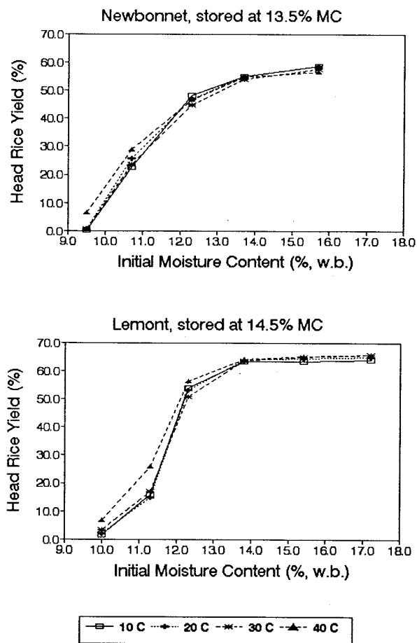
Fig. 5. Head rice yield vs. initial moisture content for the stored Newbonnet and Lemont varieties at several soaking water temperatures. Each data point is the average of head rice yields from the soaking durations in which no further head rice yield reduction occurred. Initial moisture content values are the average of 4,000 kernel moisture contents.
