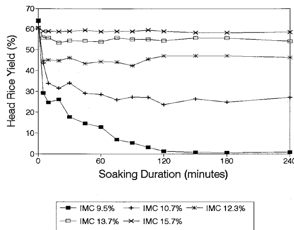
Fig. 4. Head rice yield vs. soaking duration for Newbonnet rice stored at 13.5% moisture content with the indicated initial moisture content (IMC) levels at 20°C soaking water temperature. Each data point is the average of two head rice yield determinations.
