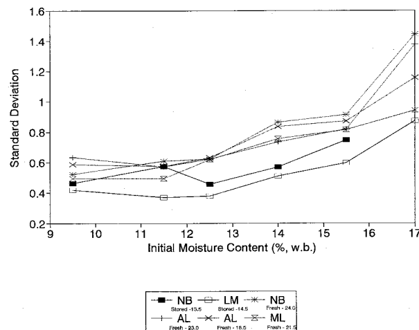
Fig. 3. Effect of initial moisture content on individual kernel moisture content standard deviations for the rice varieties Newbonnet (NB), Lemont (LM), Millie (ML), and Alan (AL), stored and fresh, at different moisture contents.
