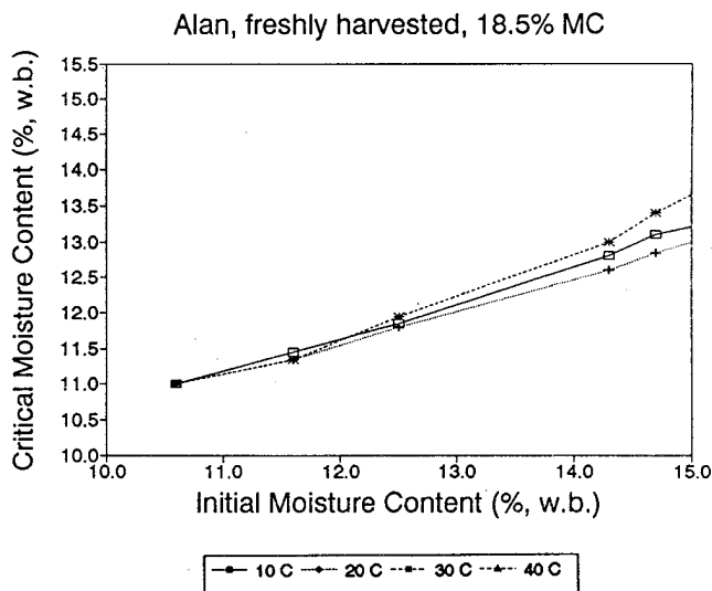
Fig. 8. Kernel critical moisture content vs. sample initial moisture content for rice and storage condition combinations at the indicated soaking water temperatures. Initial moisture content (MC) values are the average of 4,000 kernel moisture contents.
