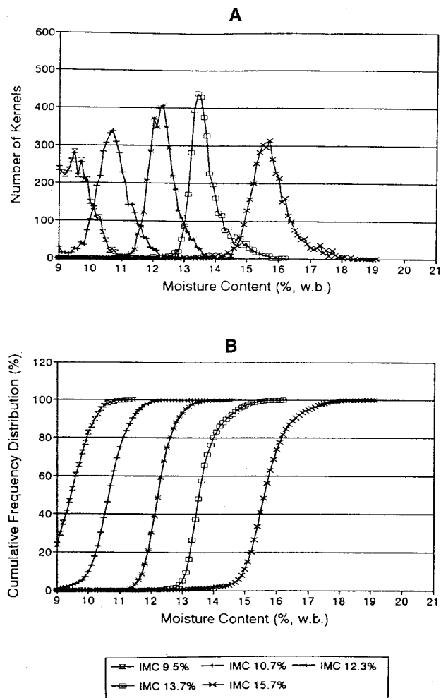
Fig. 2. Kernel moisture content frequency distributions (A) and cumulative frequency distributions (B) for 4,000-kernel samples of Newbonnet rice stored at 13.5% moisture content at five initial moisture content (IMC) levels.
