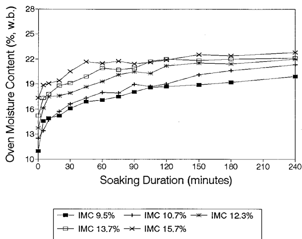
Fig. 1. Moisture adsorption curves resulting from soaking (at 20°C) Newbonnet rice stored at 13.5% moisture content with different initial moisture contents (IMC) levels.
